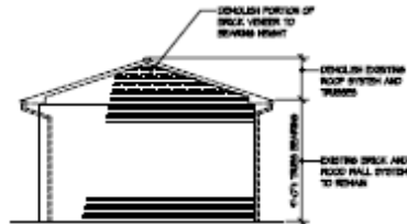
C BUILDING ELEVATION - RIGHT SCALE: 1/4" = 1'-0"
