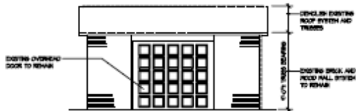
A BUILDING ELEVATION - FRONT SCALE: 1/4" = 1'-0"
