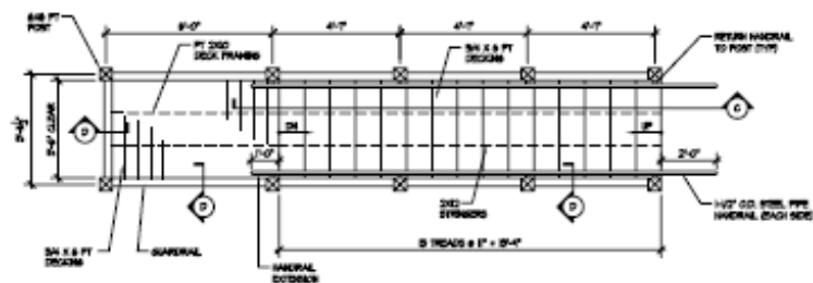
B STAIR PLAN SCALE 1/2" = 1'-0"
