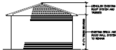
D BUILDING ELEVATION - LEFT SCALE: 1/4" = 1'-0"
