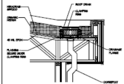
A DRAINAGE SECTION SCALE: 1/2" = 1'-0"
