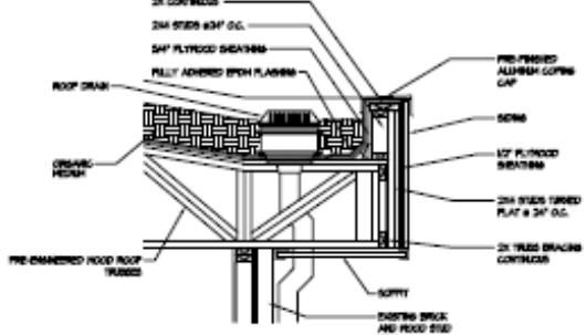
3 ROOF DETAIL SCALE: 1/2" = 1'-0"
