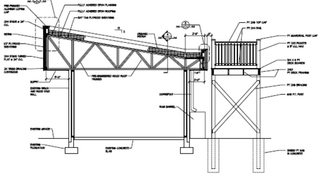
1 BUILDING SECTION SCALE: 1/2" = 1'-0"
