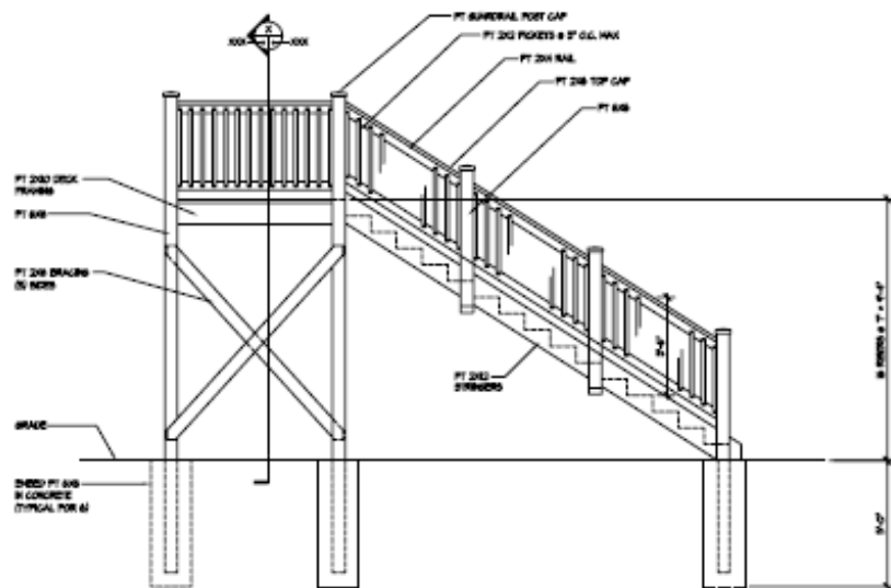
A STAIR ELEVATION SCALE 1/2" = 1'-0"
